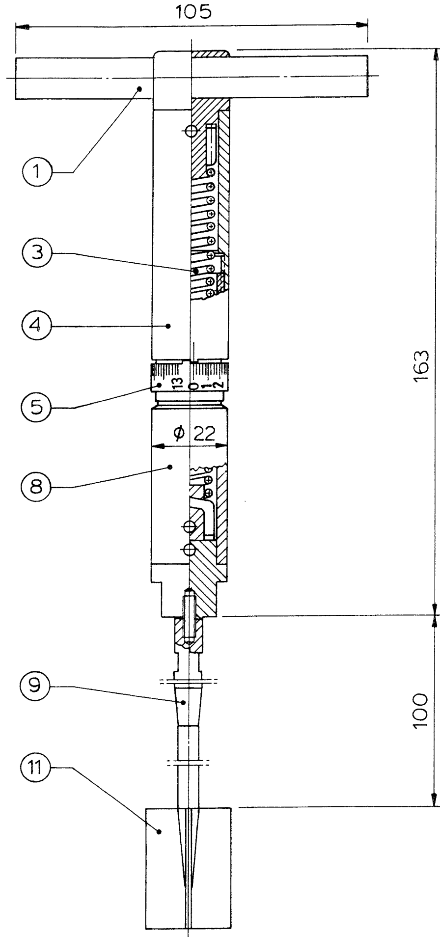
Inspection Vaneborer
